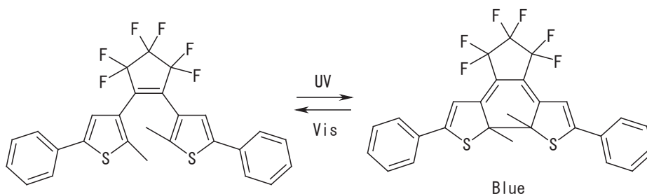
1,2-Bis(2-methyl-5-phenyl-3-thienyl) perfluorocyclopentene
