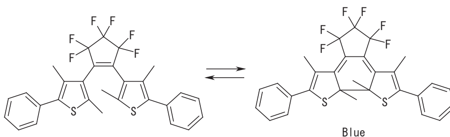
1,2-Bis(2,4-dimethyl-5-phenyl-3-thienyl) perfluorocyclopentene
