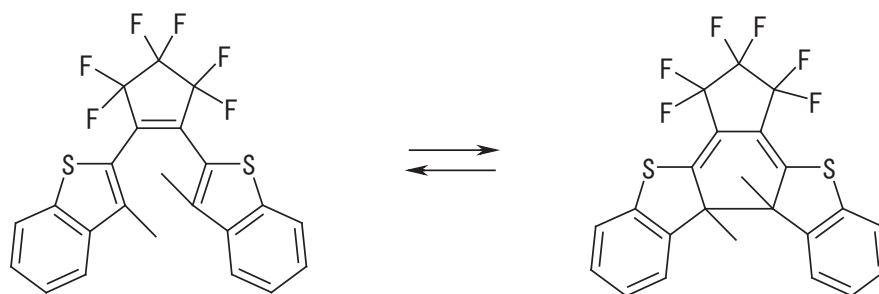
1,2-Bis(3-methylbenzo(b)thiophen-2-yl) perfluorocyclopentene
