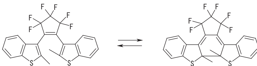
1,2-Bis(2-methylbenzo(b)thiophen-3-yl) perfluorocyclopentene
