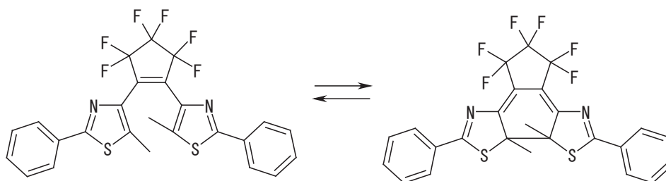
1,2-Bis(5-methyl-2-phenylthiazole-4-yl) perfluorocyclopentene
